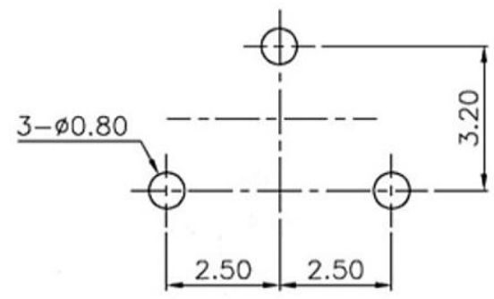
HOLE LAYOUT
